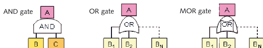
Figure 45: Schematic Fault Tree Logic Gates
