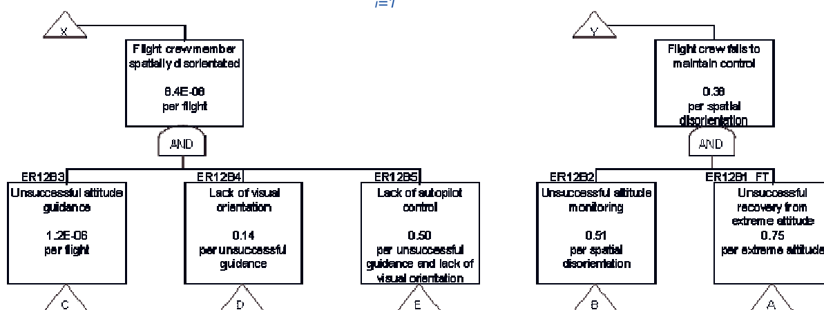
Figure 46: Top Events of Fault Tree for Spatial Disorientation
